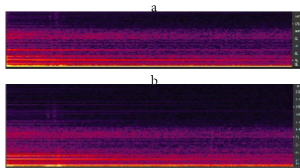
Figure 6. The spectrogram obtained from the #2 key (a) of OD and (b) of ED.
